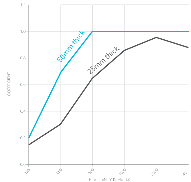
ABSORPTION DATA
